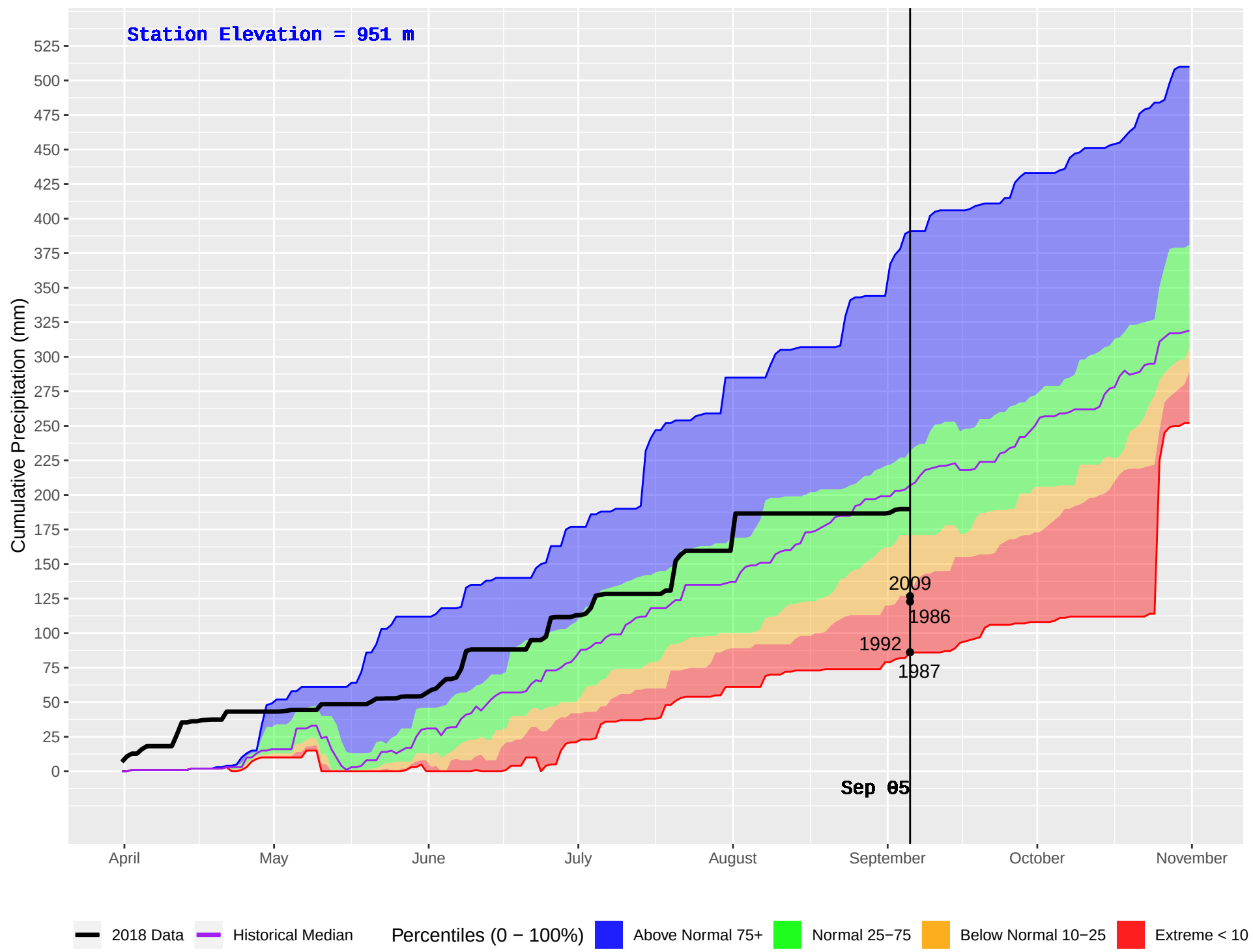
NORTH BABINE (173) : Historical (1986–2016) and Current (2018) Daily Cumulative Precipitation
