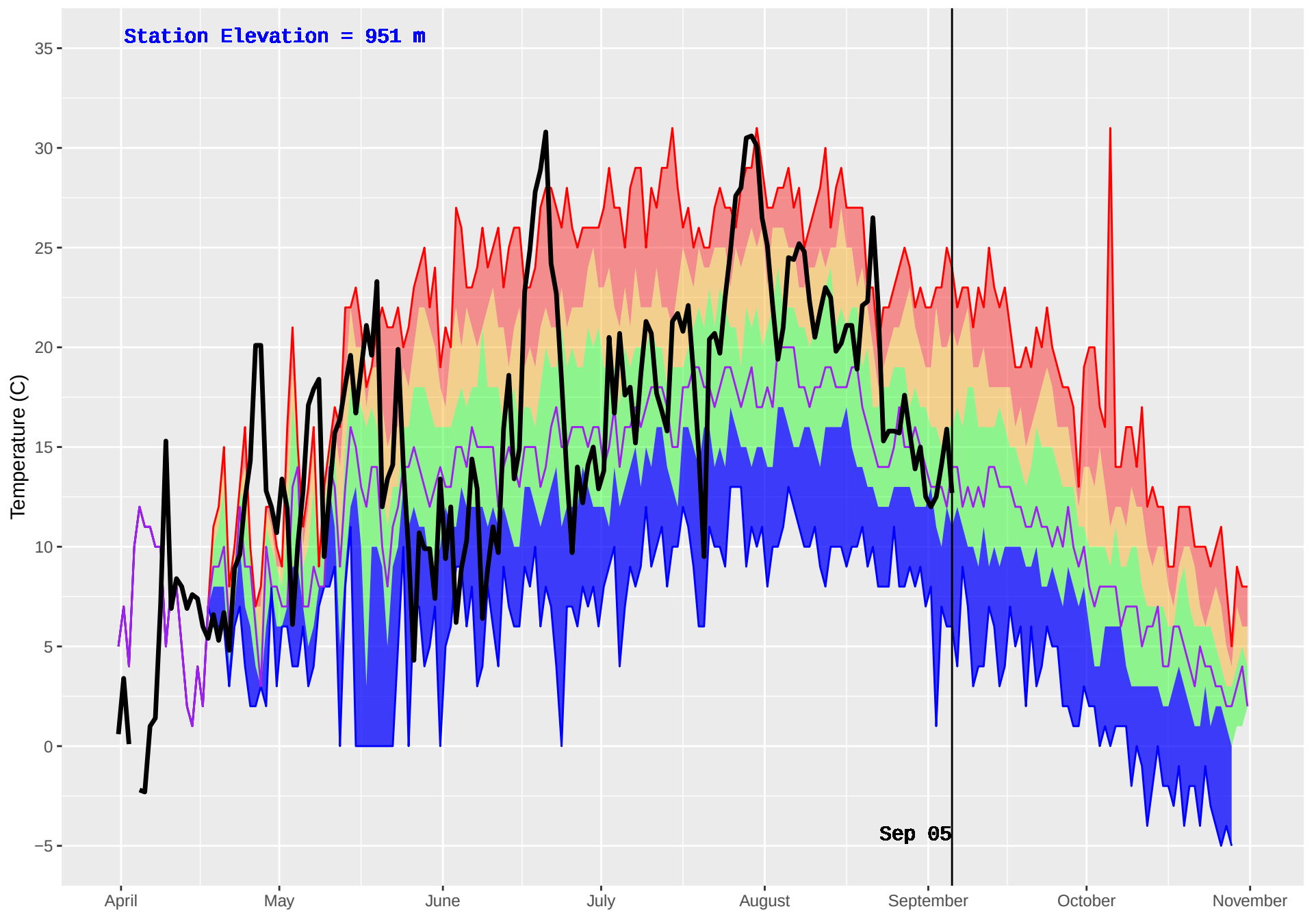
NORTH BABINE (173) : Historical (1986–2016) and Current (2018) Daily Temperature
